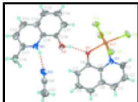
Fig. 1. The molecular structure of (I): displacement ellipsoids are drawn at the 50% probability level and H atoms are of arbitrary radius.
